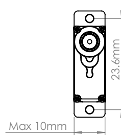
Servo type B use Frame holes B position
