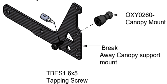
Left Canopy Mount Assembly
