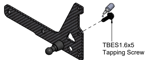
Right Canopy Mount Assembly
