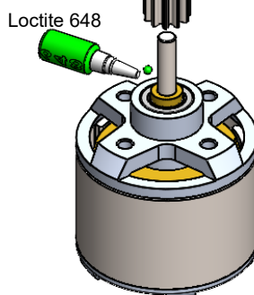
Kit Pinion 11T ID \varnothing 2mm (Box 1-1/Bag 4)
