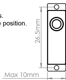
Servo type A use Frame holes A position
